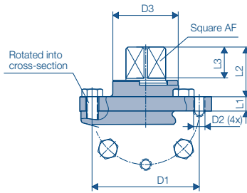
Mounting scenario with free shaft end
