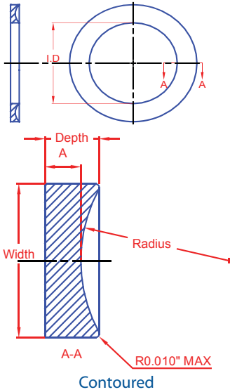
Contoured
