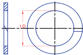
Scarf-Cut
